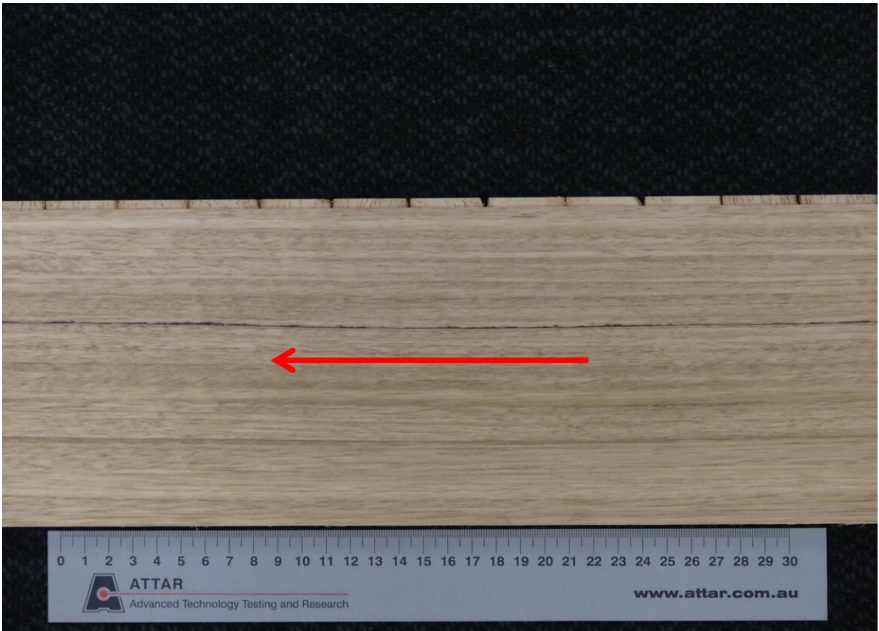
Figure 1: 14mm Engineered Timber Flooring - Eucalypt Collection Arrow indicates direction of testing
